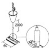
suspension câble acier
