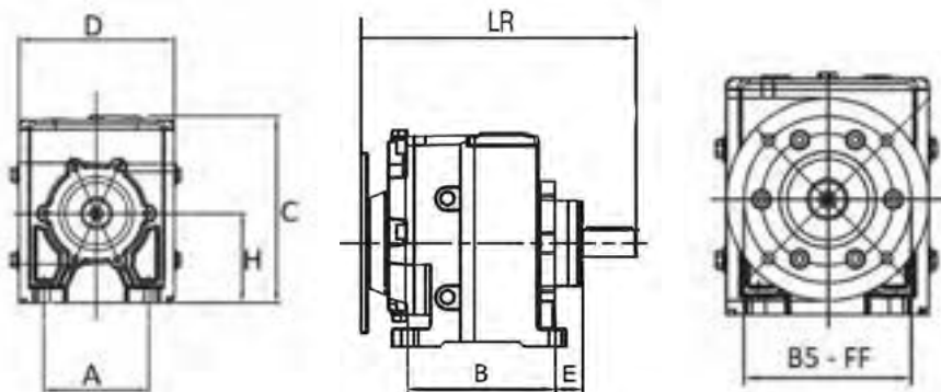
Bride B5-FF
