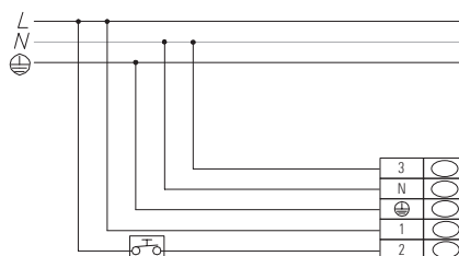
DALI - touch dim (5 core cable) 5P
