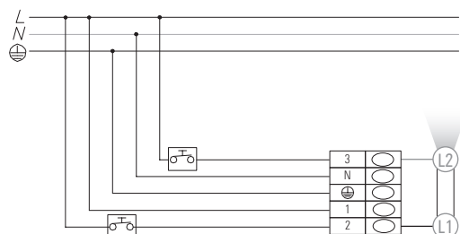
05-TD - touch dim double switch (5 core cable) 5P
