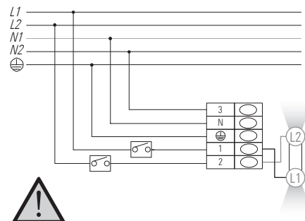
03-FO - double switch (5 core cable) 5P
