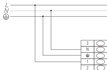
13-DALI-CASAMBI (3 core cable) 5P
